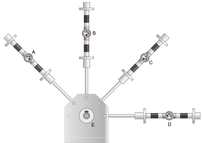
EDS-12/13: Spider for strain rosettes
