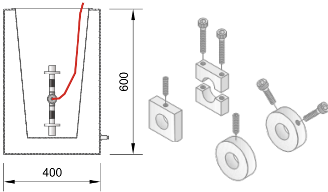
EDS-14: No stress strain container
