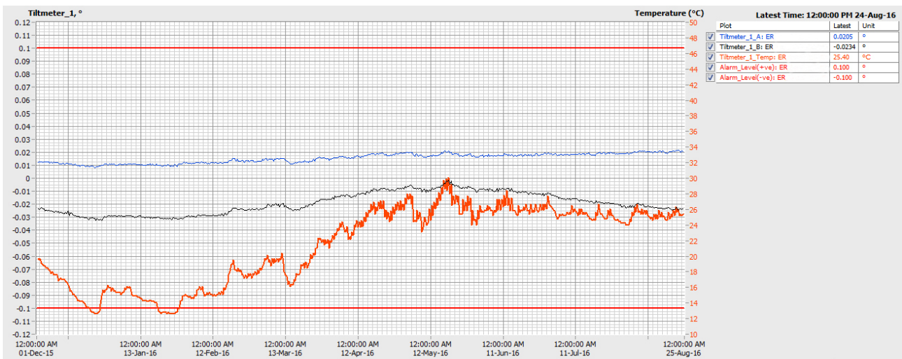
FIGURE 5: SCREEN SHOT OF GRAPH PRESENTED BY A CLOUD BASED DATA MONITORING SERVICE SHOWING EIGHT MONTHS DATA OF A BIAxIAL TILT SENSOR SAMPLED ONCE A DAY AT A FIXED TIME. THE TRACE IN RED SHOWING LARGER VARIATION IS OF AMBIENT TEMPERATURE VARIATION. THE OTHER TWO TRACES ARE MAGNITUDE OF TILT IN DEGREES ALONG TWO ORTHOGONAL AXES. THE DIFFERENCE BETWEEN THE MAXIMUM AND MINIMUM VALUE OF TILT REGISTERED IS APPROXIMATELY 0.02 DEGREES. THE TWO RED LINES AT THE TOP AND BOTTOM ARE ALARM LIMITS SET FOR THE BIAxIAL TILT SENSOR.
