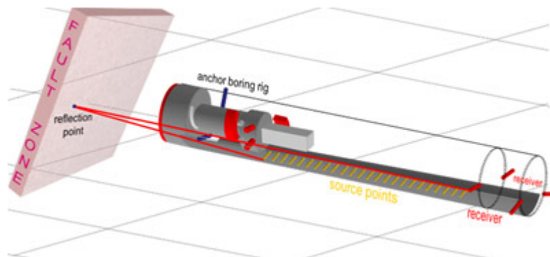
FIGURE 11 STANDARD TSP LAYOUT IN A TBM HEADING. ACOUSTIC WAVES ARE REFLECTED FROM A GEOLOGICAL DISCONTINUITY AND PICKED UP BY RECEIVERS
