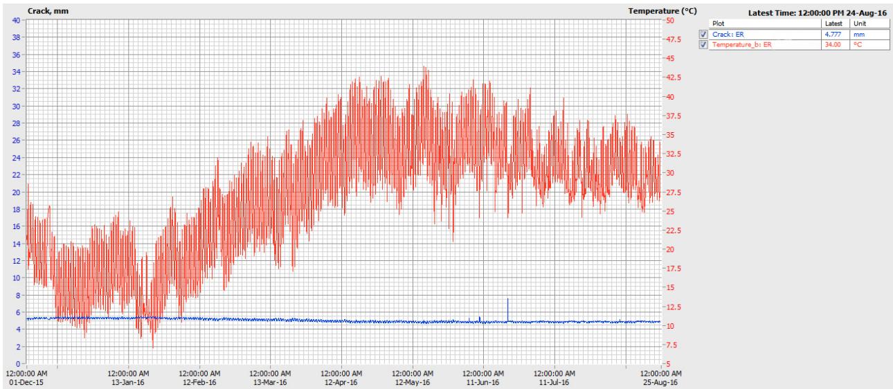
FIGURE 6: SHOWS EIGHT MONTHS DATA OF CRACK METER SET AT 6 MM TO REGISTER BOTH CLOSING AND OPENING OF CRACK WITH TIME. BAND LIKE TRACE IS AMBIENT TEMPERATURE. AS SENSOR IS BEING SAMPLED EVERY 30 MINUTES IT IS TRACKING VARIATION IN AMBIENT TEMPERATURE OVER WHOLE DAY UNLIKE FIGURE 5 IN WHICH SENSOR IS SAMPLED ONCE A DAY.
