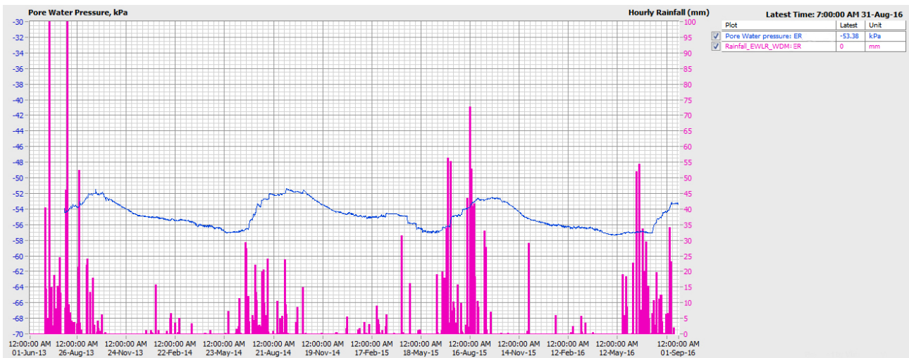
FIGURE 7: SHOWS THREE YEAR'S DATA OF CHANGES IN GROUND WATER TABLE AND RAINFALL. GROUND WATER LEVEL IS LOGGED FOUR TIMES A DAY. RAINFALL IS LOGGED CONTINUOUSLY. DATA IS TRANSMITTED ONCE A DAY TO CLOUD SERVER. CO-RELATION OF VARIATION IN GROUND WATER LEVEL WITH RAINFALL CAN BE SEEN ON THE GRAPH. SIMILAR INSTRUMENTATION IS USED FOR ONLINE AUTOMATIC MONITORING OF RIVER WATER LEVEL AND RAINFALL WITH TIME.
