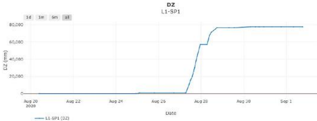
Figure 4 : Graph showing change in elevation of the Link Bridge during its lifting procedure
