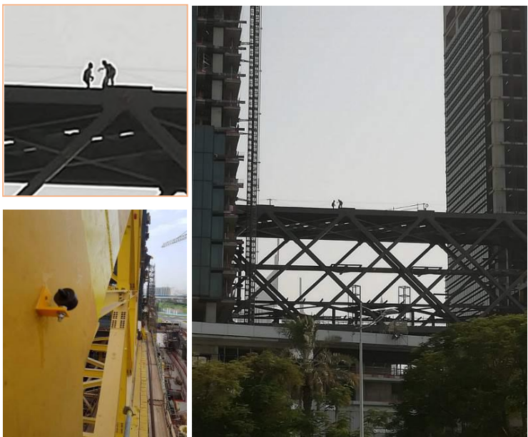
Installation of the prism targets on the Link Bridge
