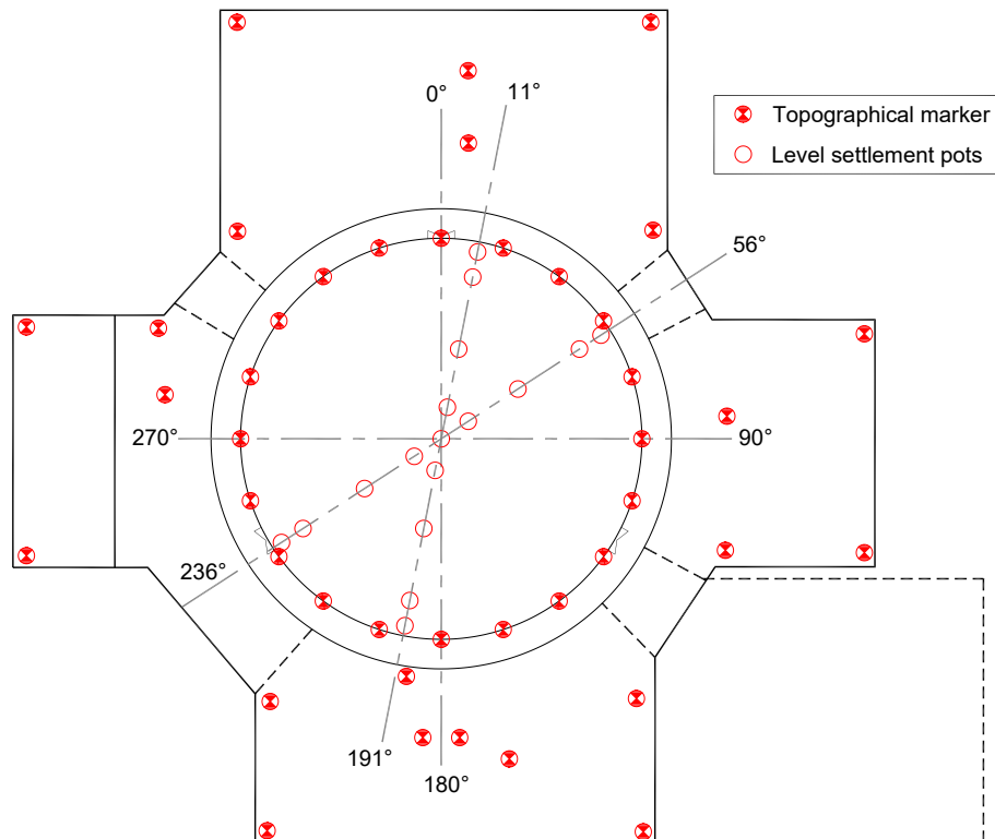
Typical locations of topographical markers and hydraulic settlement system pots in the raft
