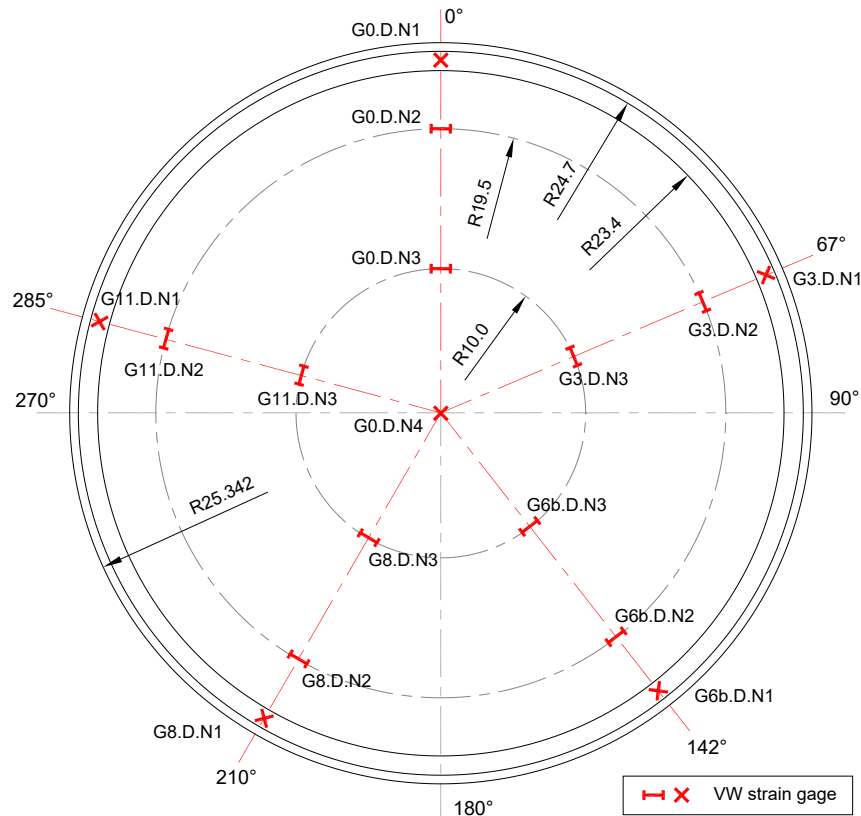
Typical location of strain gages at the common raft
