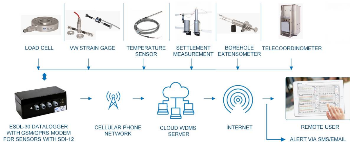
Remote real-time monitoring system with SDI-12 digital interface sensors and dataloggers
