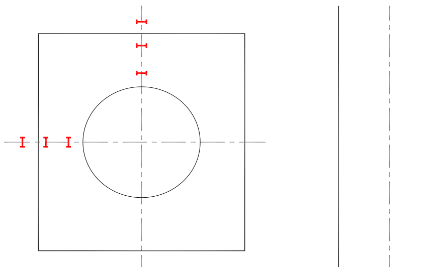
Typical location of strain gages in the equipment hatch
