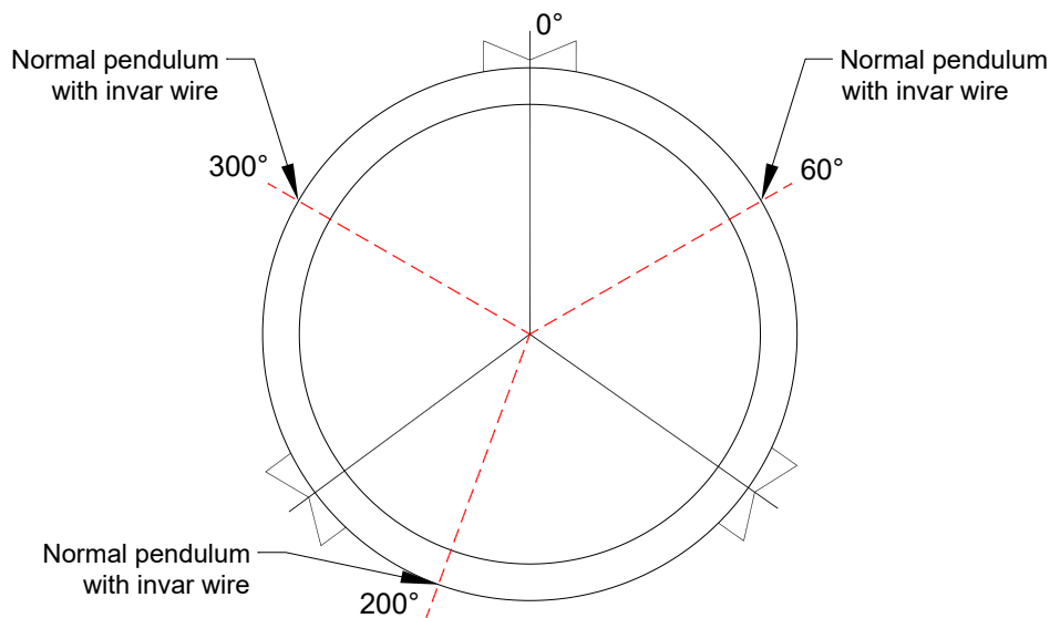
Typical locations for the normal plumb lines with invar wire
