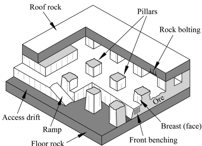
Room & pillar mining
