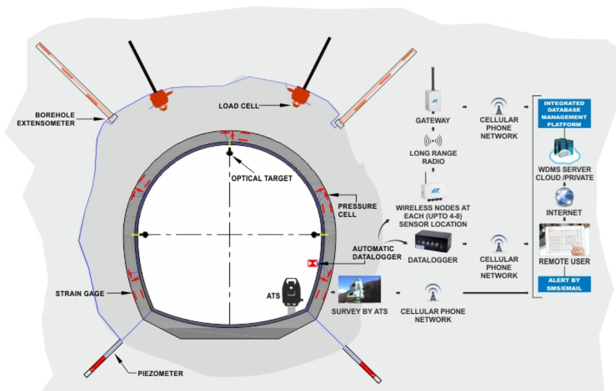
Typical monitoring plan for underground mine/cavern
