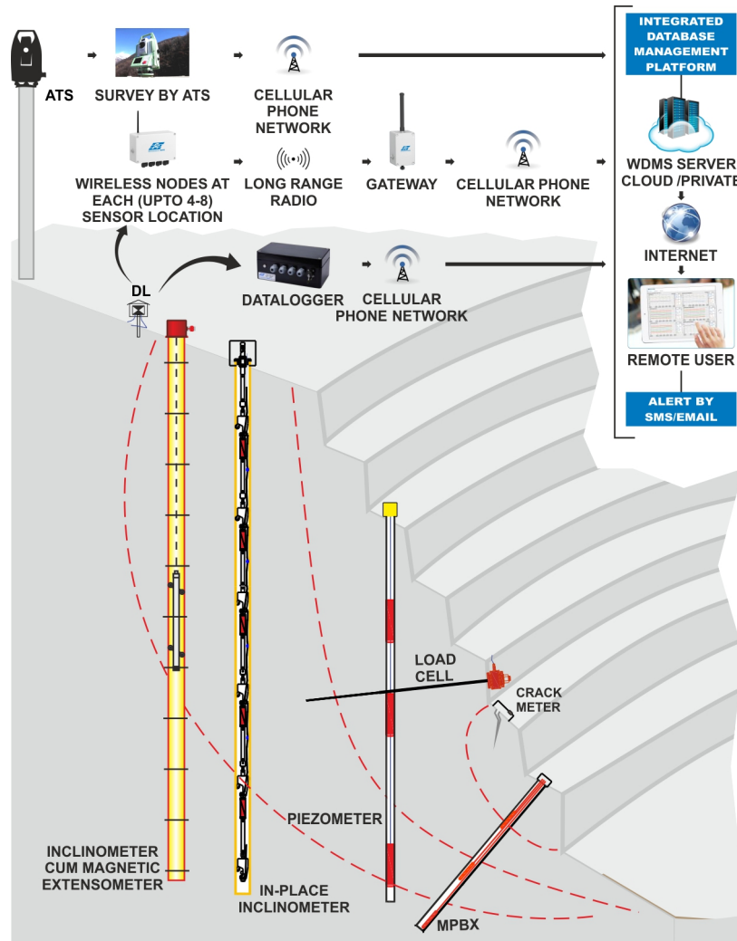
Typical monitoring plan for Open-pit mines
